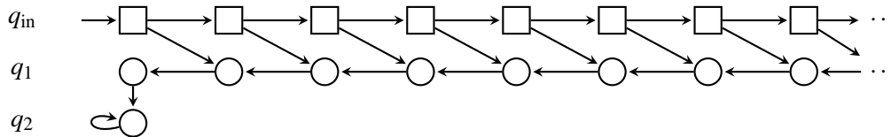
Figure 1: A pushdown game graph (only the part reachable from the initial vertex is shown)
